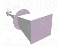
LB-62-25-C2-TFSPO Standard Gain Horn Antenna 12.4-18GHz 25dB Gain TNC Female
